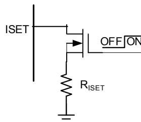
Figure 4— ISET Logic Control
