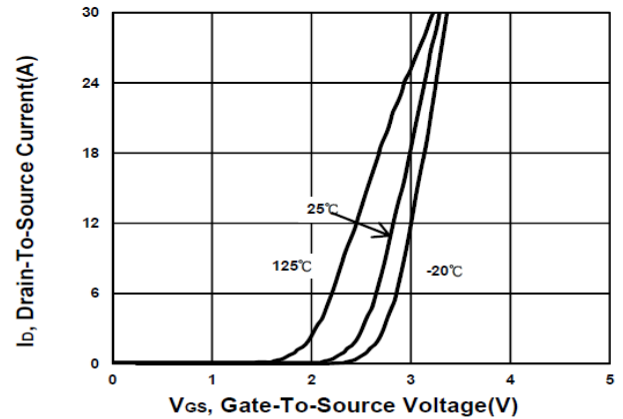
Transfer Characteristics
