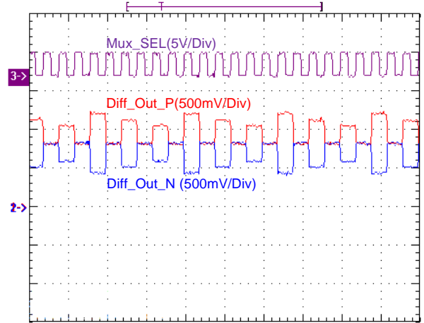
Time : 40us/Div
