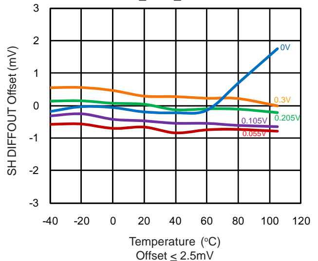
Shunt_DIFF_OUT Offset
