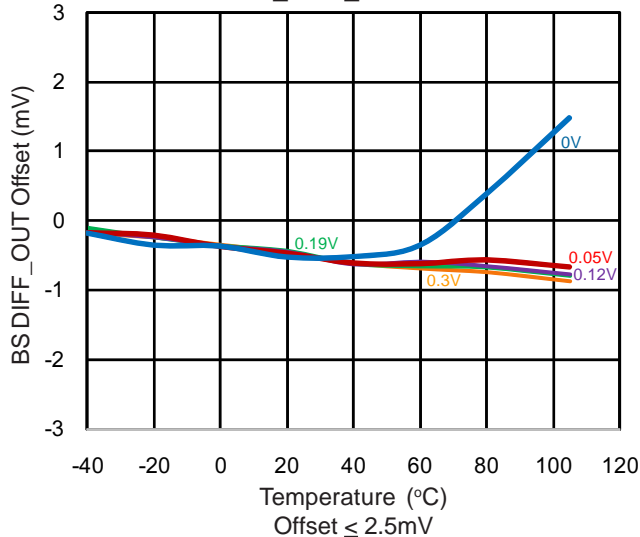
BUS_DIFF_OUT Offset
