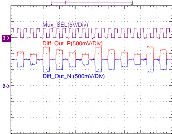
Time : 40us/Div
