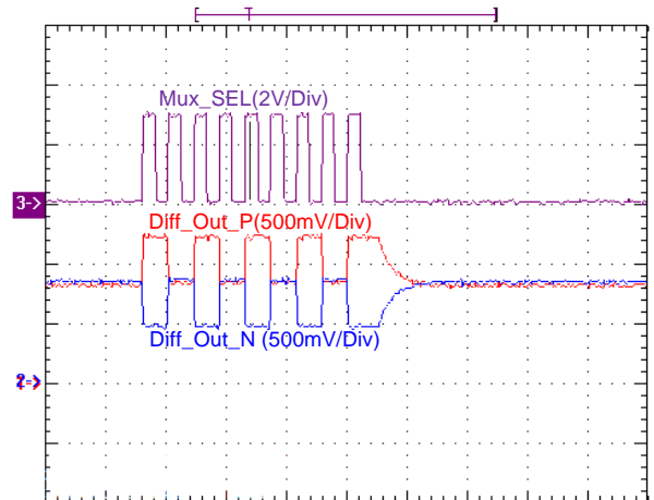
Time : 100us/Div
