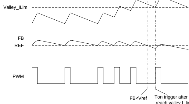
Figure 7: Valley Current-Limit Operation
