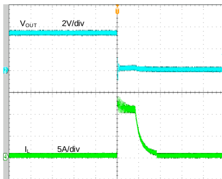
Output Short Circuit Protection ( V_N=12V , V_{OUT}=3.338V , I_{OUT}=0A -Short)
