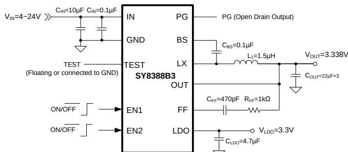
Figure1. Schematic Diagram
