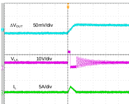
Output Ripple ( V_N=12V , V_{OUT}=3.338V , I_{OUT}=0A , PFM)
