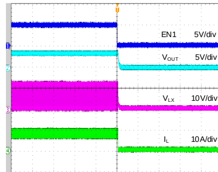
Shutdown from EN1 ( V_N=12V , V_{OUT}=3.338V , I_{OUT}=8A )
