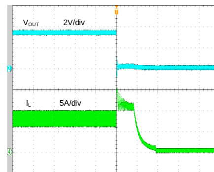
Output Short Circuit Protection ( V_N=12V , V_{OUT}=3.338V , I_{OUT}=8A -Short)
