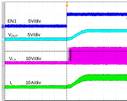
Startup from EN1 ( V_N=12V , V_{OUT}=3.338V , I_{OUT}=8A )
