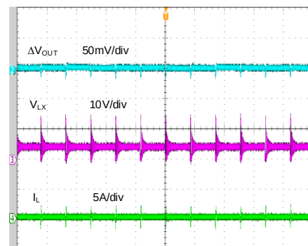
Output Ripple ( V_N=12V , V_{OUT}=3.338V , I_{OUT}=8A , USM)
