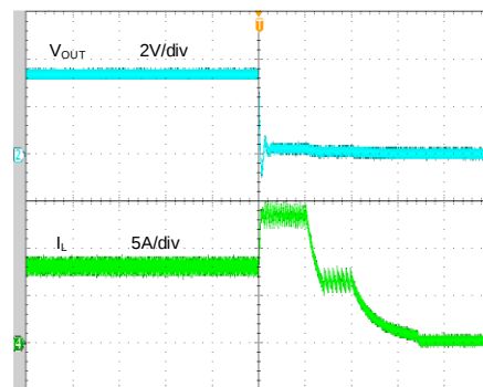
Output Short Circuit Protection ( V_{IN}=12V , V_{OUT}=3.338V , I_{OUT}=8A ~Short)
